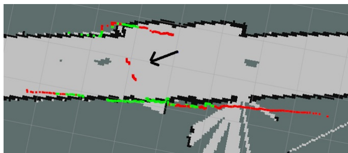
Fig. 11. Illustration of the sensor model P(z_t | x_t, M) for a given position of the robot. The robot is located at the origin of the arrow and the arrow shows its orientation. Green points are hits of the laser that match to an occupied cell and red one are points that match to an empty cell.
